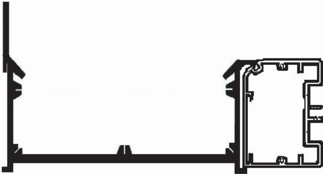
240mm Box gutter with a single ring beam attached equals 305mm
