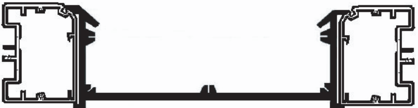
240mm Box gutter with 2x ring beams attached equals an overall dimension of 370mm
